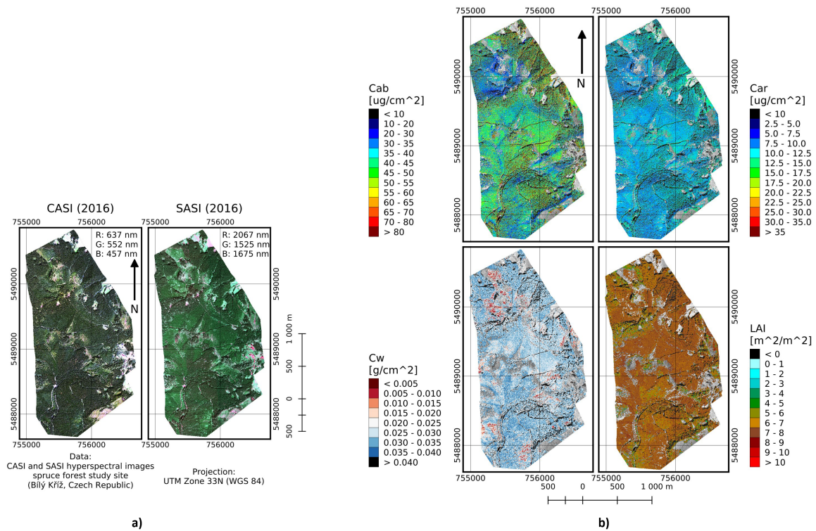
Figure 5: Vegetation trait retrieval workflow. Left: True-color (CASI 2016) and false-color (SASI 2016) hyperspectral images of a forest study site. Right: Retrieved trait maps showing spatial distribution of leaf chlorophyll content (Cab), leaf carotenoids content (Car), leaf water content (Cw), and leave area index (LAI). Color scales indicate concentration gradients across the heterogeneous canopy. Source: Janoutová et al. (2021).
