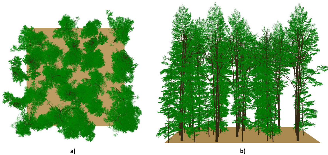
Figure 11: 3D forest scene representation in DART. (a) Top-down view showing tree positions in systematic grid pattern with brown ground visible between crowns. (b) Oblique 3D view showing detailed tree architecture with individual crowns, trunks, and branches. Scene dimensions are 30m × 30m with trees positioned to achieve target canopy cover and LAI. Source: Hanousek et al. (2024).
