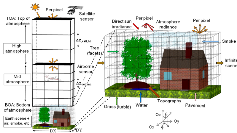
Figure 2: Canopy-level radiative transfer in 3D scene. The diagram shows the DART model structure including atmosphere layers (high and mid atmosphere), Earth scene with detailed 3D vegetation (trees, grass, water, topography), and multiple sensor configurations. Key elements include: TOA (Top of Atmosphere), BOA (Bottom of Atmosphere), direct sun irradiance, atmosphere radiance, per-pixel radiation, and both satellite and airborne sensor geometries. Source: Gastellu-Etchegorry et al. (2017).
