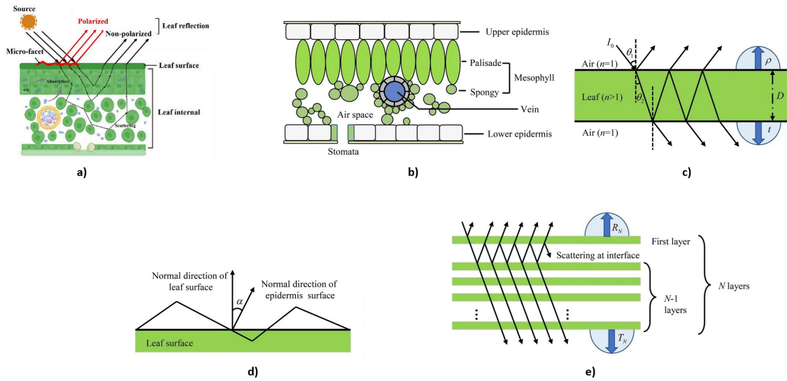
Figure 1: Leaf-level radiative transfer mechanisms. (a) Light interaction with leaf structure: polarized (red) and non-polarized (black) light interact through surface reflection at micro-facets, absorption by chloroplasts, and scattering within mesophyll tissue. (b) Conceptual diagram showing light interaction with leaf surface and internal structures including epidermis, palisade, spongy mesophyll, and air spaces. (c) Simplified plate model showing light transmission and reflection through mesophyll layers with refractive index n > 1 . (d) Detailed representation of light path including surface reflection and internal scattering at multiple interfaces. (e) Multi-layer representation with N layers showing transmittance ( T_N ) and reflectance ( R_N ) terms. Sources: (a) Li et al. (2025), (b) Xu and Ye (2023).
