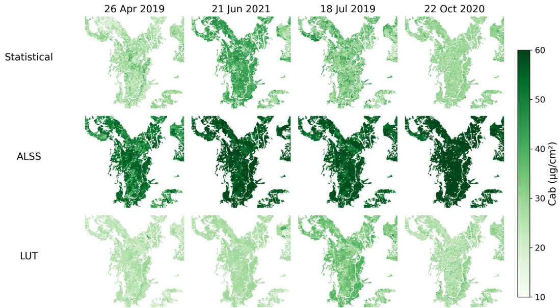
Figure 14: Comparison of retrieval methods on seasonal hyperspectral imagery. Three rows show results from Statistical (empirical regression), ALSS (Adaptive LUT Subset Selection), and LUT (full Look-Up Table matching) methods. Four columns represent different dates: 26 Apr 2019, 21 Jun 2021, 18 Jul 2019, and 22 Oct 2020. Color scale shows chlorophyll content (Cab) from 10-60 \mu\text{g}/\text{cm}^2 . All methods capture seasonal variation (low chlorophyll in spring/autumn, high in summer) and spatial patterns (individual tree crowns), but differ in smoothness and detail. ALSS balances accuracy and robustness. Source: Slanínáková et al. (2025).
