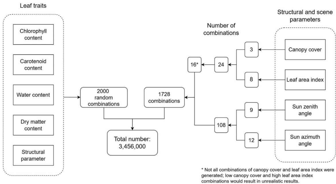
Figure 12: Look-Up Table generation strategy. Flow diagram shows how leaf traits (chlorophyll, carotenoids, water, dry matter, structural parameter) combine with structural and scene parameters (canopy cover, LAI, sun zenith angle, sun azimuth angle). Total possible combinations: 3.5 million. Through random sampling (2000 combinations) and filtering for realism (1728 combinations remain after excluding unrealistic scenarios like low canopy cover with high LAI), these are organized into trait groups, then expanded across structural-geometric combinations, yielding a final database of 3,456,000 spectra. Source: Hanousek et al. (2024).
