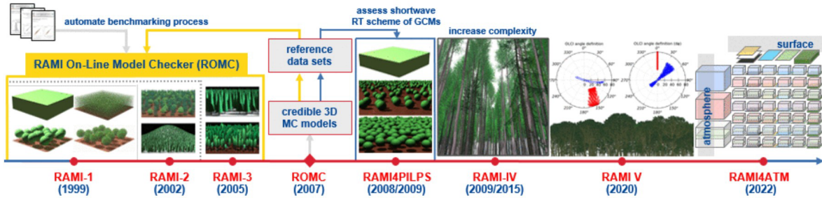
Fig 1: the figure shows all RAMI phases from the beginning (evolution from 1999 until 2022). @Copyright
