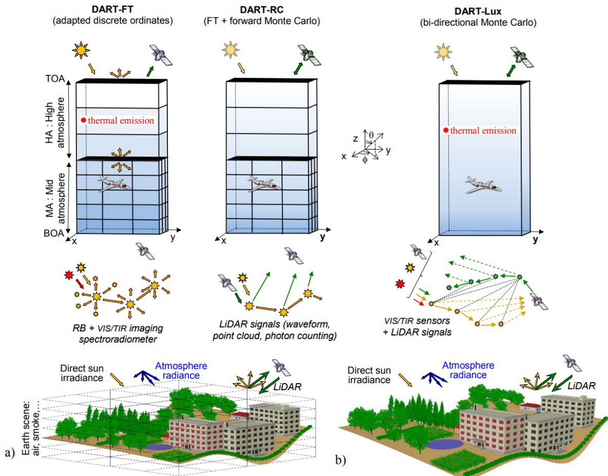
Figure 8: DART model architecture showing three computational modes. Left: DART-FT using adapted discrete ordinates with voxelized atmosphere and scene. Center: DART-RC using forward Monte Carlo ray tracing with photon tracking. Right: DART-Lux using bi-directional path tracing with explicit triangle meshes. All modes simulate optical, thermal, and LiDAR products for natural and urban landscapes. Source: DART User Manual - https://dart.omp.eu/Public/documentation/contenu/documentation/DART_User_Manual.pdf
