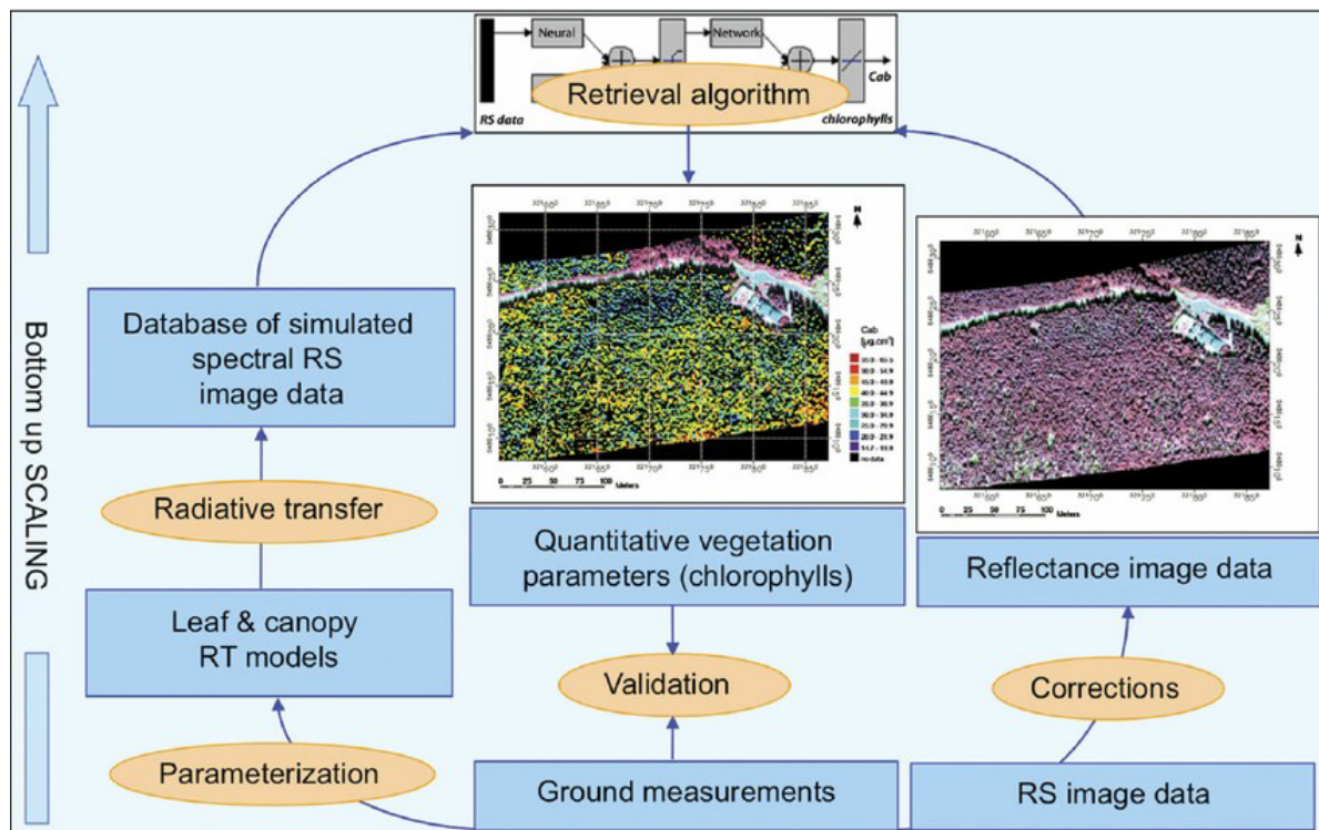
Figure 9: Vegetation traits retrieval workflow. The process flows from bottom to top: (1) Leaf & canopy RT models are parameterized with ground measurements, (2) Radiative transfer simulations generate a database of spectral signatures for quantitative vegetation parameters (chlorophylls shown as example), (3) Retrieval algorithm compares this database with reflectance image data (after corrections), (4) Validation using ground measurements confirms accuracy. The workflow represents bottom-up scaling from leaf to canopy level. Source: Malenovsky et al. (2009).
