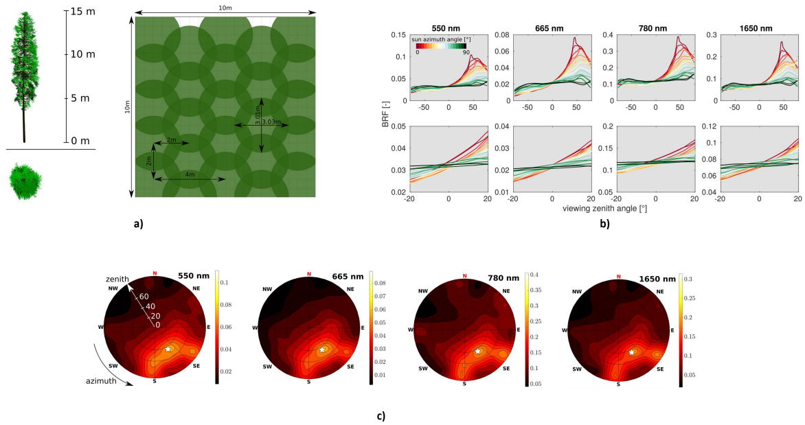
Figure 4: Multi-angle BRF patterns for a forest canopy. Polar plots showing BRF at four wavelengths (550 nm, 665 nm, 780 nm, 1650 nm) across viewing hemisphere. (a) Canopy simulation design. (b) BRF vs. viewing zenith angle for different solar positions (shown as colored lines). (c) Polar projections with solar position marked by star symbol. Patterns reveal strong forward scattering (hotspot) and angular anisotropy varying with wavelength. Source: Hanuš et al. (2023).
