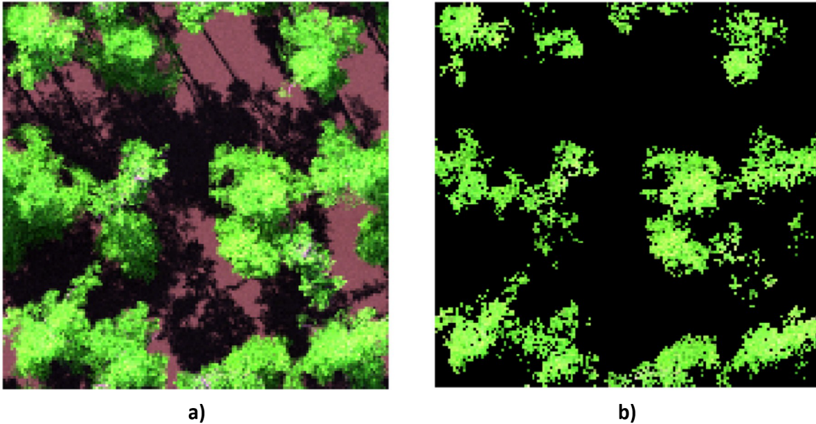
Figure 13: Processing of simulated DART imagery. (a) RGB composite showing forest canopy with green sunlit leaves, dark shadows between crowns, and brown/purple mixed pixels at crown edges. (b) Binary mask isolating only sunlit leaf pixels (bright green) while excluding shadows, woody parts, and ground. This masking ensures that LUT spectra represent the same surface types as pixels used in retrieval from real imagery. Source: Hanousek et al. (2024).
