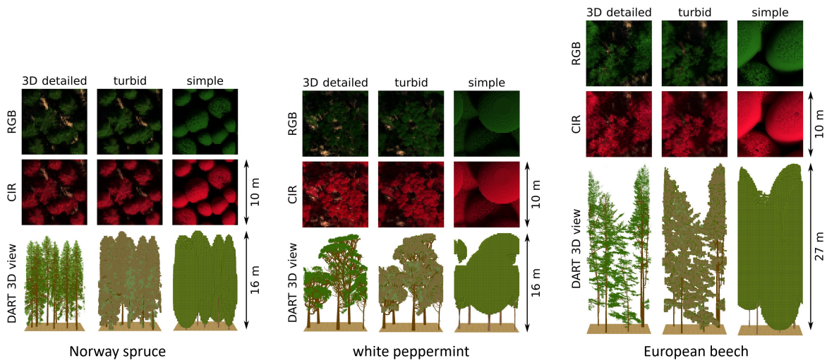
Figure 6: Sensitivity analysis for different tree types and canopy representations. Simulated RGB, CIR (Color Infrared), and 3D canopy views for three species (Norway spruce, white peppermint, European beech) using three modeling approaches: 3D detailed, turbid medium, and simple geometric representation. Each representation creates different spatial patterns and spectral responses, revealing the importance of architectural fidelity for accurate simulations. Source: Janoutová et al. (2021).
