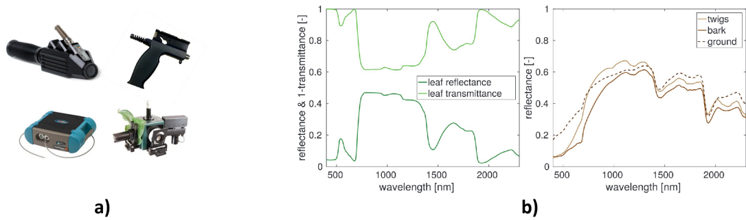
Figure 10: Field measurement equipment and spectral data. (a) Spectroradiometers with contact probe (bark), pistol grip (ground), and integrating sphere (leaves). (b) Example spectral reflectance and transmittance curves for leaves (green wavelengths show characteristic chlorophyll absorption), and reflectance spectra for twigs/bark (brown) and ground (dashed black). These field measurements provide the optical properties needed to parameterize RTMs.
